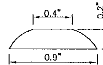
SECTION OF DOME FROM A DETECTABLE WARNING. DRAWING SHOWS HEIGHT, TOP AND BOTTOM DIMENSIONS
