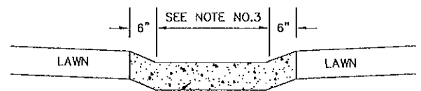
CONCRETE CURB RAMP, 6" THICK
