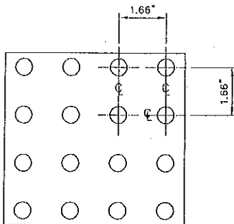
PLAN AND SECTION VIEWS OF DETECTABLE WARNING DOMES AND THEIR RELATIVE SPACING ON THE X AND Y AXIS
