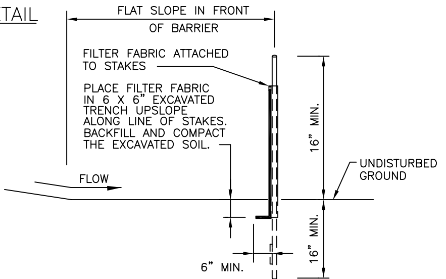
SILT FENCE SECTION NO SCALE
