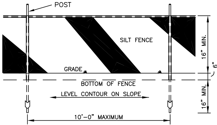
SILT FENCE DETAIL NO SCALE
